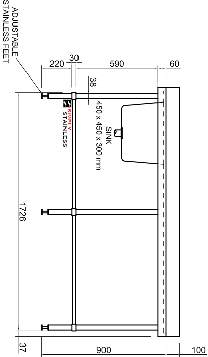
FRONT ELEVATION
