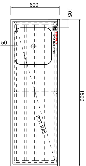
PLAN
