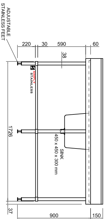
FRONT ELEVATION
