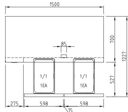
PLAN VIEW
