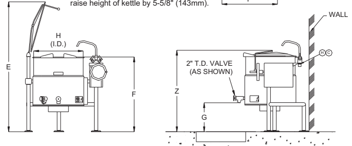
KETTLE SHOWN WITH OPTIONAL SPRING ASSIST COVER, WATER FAUCET AND T.D. VALVE
