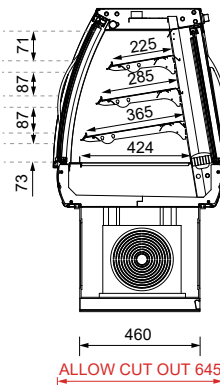
SECTION VIEW
