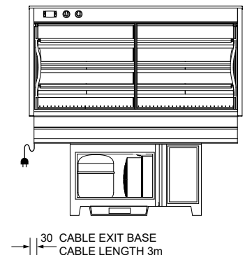
REAR ELEVATION
