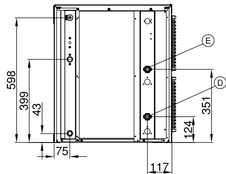
WATER COOLED
