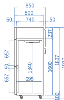
SIDE VIEW (Half Door)
