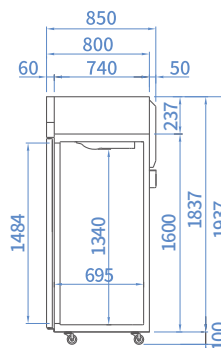
SIDE VIEW (Full Door)
