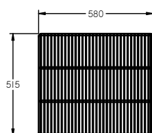
SHELF DETAIL
