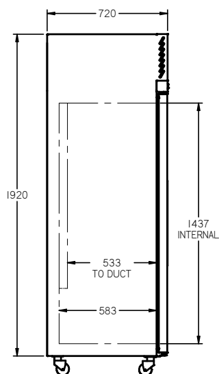
SHELF DETAIL
