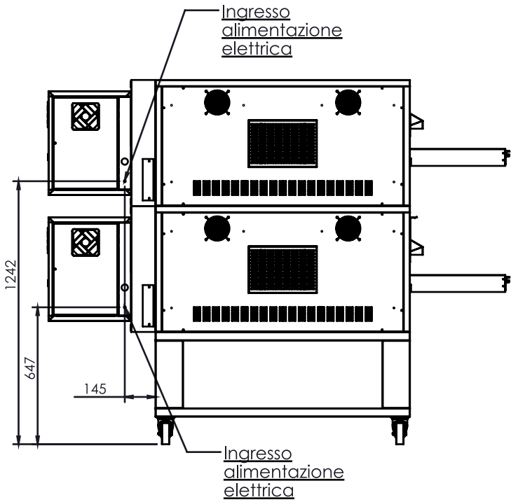
REAR
